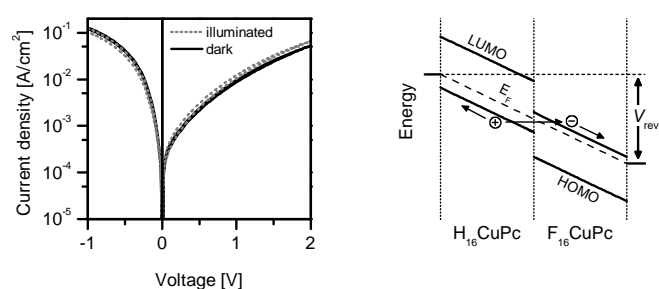
Figure 8: (left) Current-voltage characteristic for an ambipolar H_{16}CuPc/F_{16}CuPc bilayer diode in the dark and under one sun illumination. (right) Energy level diagram for an H_{16}CuPc/F_{16}CuPc bilayer diode to explain the charge generation layer under reverse bias conditions. The energy levels for H_{16}CuPc are taken from our own measurements and the energy levels for F_{16}CuPc from the literature [41].
