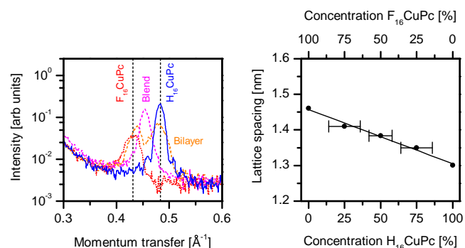
Figure 3: (left) X-ray diffraction spectra of neat films, a 1:1 blend and a bilayer structure evaporated onto PEDOT:PSS at room temperature. (right) Analysis of the lattice spacing determined from X-ray scattering spectra of films with different mixing ratios. The straight line is the linear fit of the measurement points.
