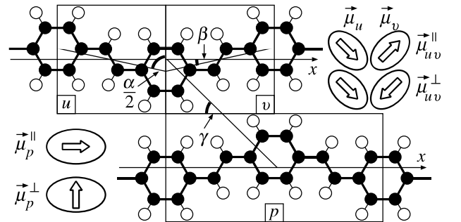
Fig. 3. Proposed intra- and intermolecular structure of trans-cisoid h-PPV. Two intrachain excitation sites u, v are shown arranged in zig-zag configuration along the chain axis x that lead to transitions (I) || , (II) ± ; p denotes localized aromatic transitions (IIIa,b) ± , (IV) || in the dimers.
