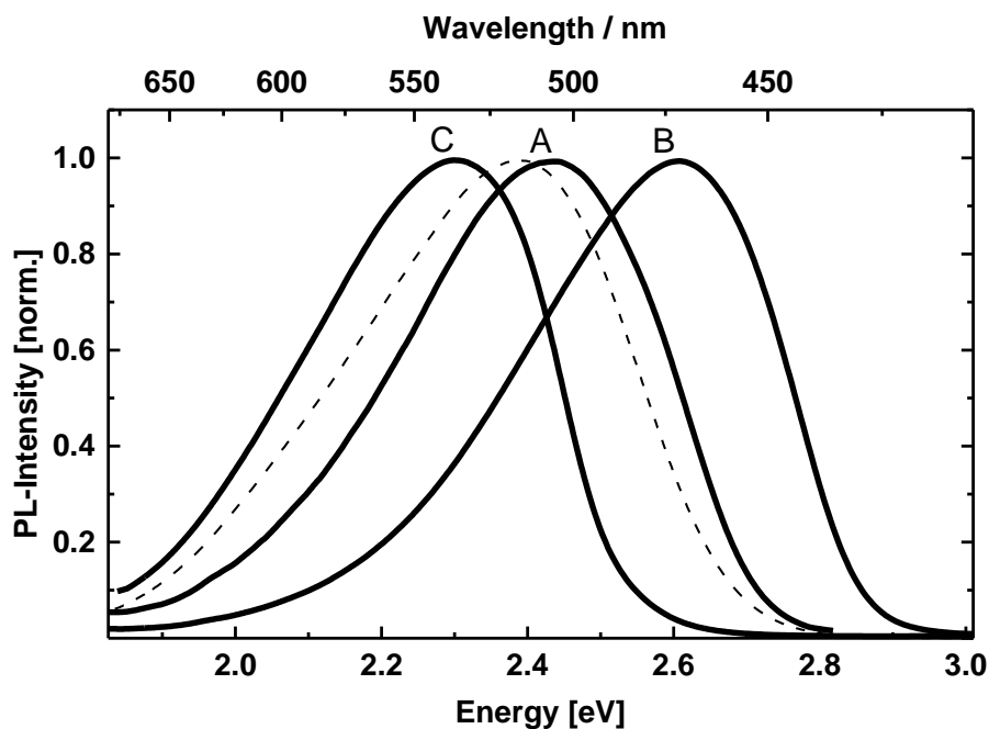
Figure 4: PL spectra of Alq 3 samples taken from the regions A, B and C of Figure 3 respectively, excited at 350nm. For comparison the PL of an evaporated Alq 3 film is shown (dashed line).
