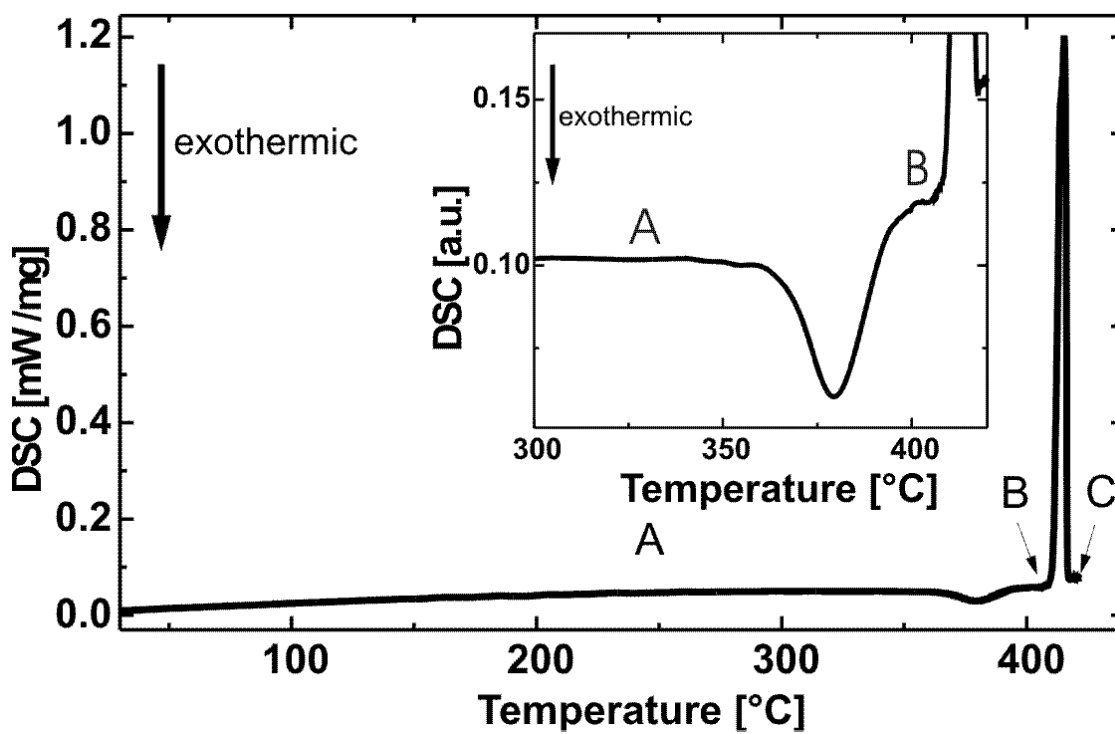
Figure 3: DSC trace of Alq 3 measured with a heating rate of 2°C/min. The clearly pronounced exothermic phase transition at 380°C prior the melting point is zoomed out in the inset, as it becomes broad and less intense with respect to the melting peak for this slow heating rate. A, B and C mark the regions of yellowish-green Alq 3 , blue Alq 3 and melt, respectively.
