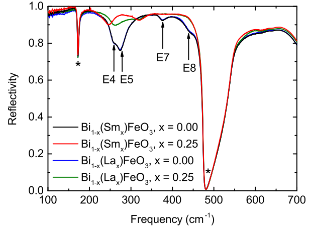
FIG. 2. Reflectivity of undoped ( x=0 ) and maximum doped ( x=0.25 ) \text{BiFeO}_3 films. The strongest modes of \text{BiFeO}_3 are labeled according to the literature. 28 The strong features around 172\text{ cm}^{-1} and 481\text{ cm}^{-1} marked with asterisks are due to excitations in the STO substrate. 30–32
