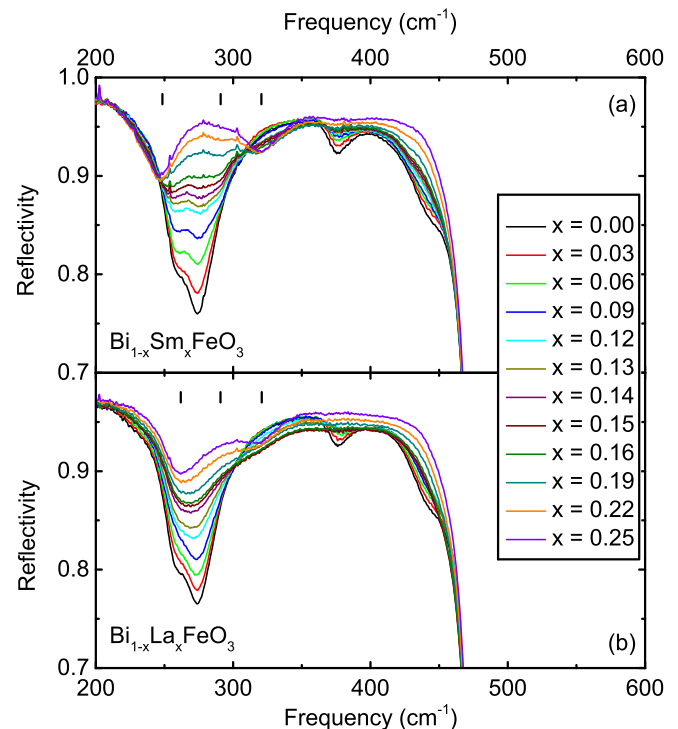
FIG. 3. Evolution of the reflectivity with increasing dopant content for (a) \text{Bi}_{1-x}\text{Sm}_x\text{FeO}_3 and (b) \text{Bi}_{1-x}\text{La}_x\text{FeO}_3 . The ticks mark the three strongest modes for maximum doping x=0.25 in both cases.
