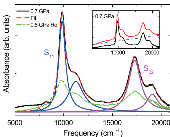
Figure 3 Data evaluation of the absorbance spectra: illustration of the fitting procedure of the spectrum with Lorentzians corresponding to the S_{11} and S_{22} optical transitions. Also, the spectrum at 0.8 GPa after pressure release is plotted. The inset illustrates the subtraction of a linear background (dashed line).
