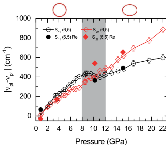
Figure 4 Relative energy shift of the optical transitions as a function of pressure in (6,5)-SWCNTs. The shift was calculated as the difference between the absorption frequency of the contribution \nu_{p_i} at a pressure p_i , and the absorption frequency \nu_{p_1} at the lowest pressure value p_1 . All the contributions during pressure release are marked as S_{ij} (Re). The shaded gray bar marks the critical pressure regime as discussed in the text. The proposed structural deformation is illustrated on the top.
