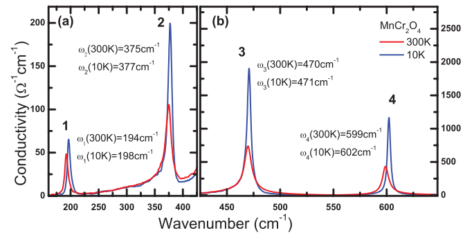
FIG. 3. (Color online) Optical conductivity spectra of MnCr_2O_4 at T = 300 and 10 \text{ K} contain four distinct phonon modes. Neither the ferrimagnetic transition at T_C = 51 \text{ K} nor the onset of conical spin order at T_S = 14 \text{ K} are accompanied with an observable splitting of these T_{1u}(\text{IR}) phonon modes. Note that the conductivity scales for panels (a) and (b) differ by more than an order of magnitude.
