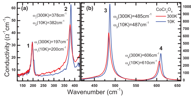
FIG. 4. (Color online) Optical conductivity spectra of \text{CoCr}_2\text{O}_4 at T = 300 and 10 K. Similarly to \text{MnCr}_2\text{O}_4 , no splitting of the four T_{1u} (IR) phonon modes can be traced either below the ferrimagnetic transition at T_C = 93 K or upon the conical spin ordering at T_S = 26 K.
