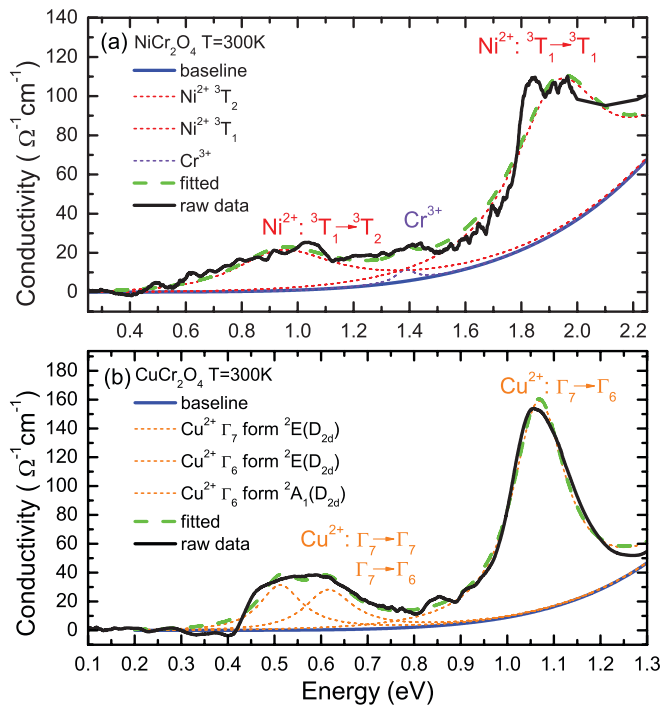
FIG. 11. (Color online) Analysis of the intra-atomic 3d - 3d transitions in NiCr_2O_4 and CuCr_2O_4 as shown in panels (a) and (b), respectively. Labels correspond to notation introduced in Fig. 10. Aside from the oscillators, there is a common baseline corresponding to the tail of the band edge.
