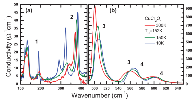
FIG. 8. (Color online) Optical conductivity spectra of \text{CuCr}_2\text{O}_4 at various temperatures. At room temperature, all T_{1u} (IR) phonon modes are split due to the Jahn-Teller transition at T_{JT} = 854 K. For each mode, the remaining degeneracy is lifted upon the magnetic ordering at T_C = 152 K.
