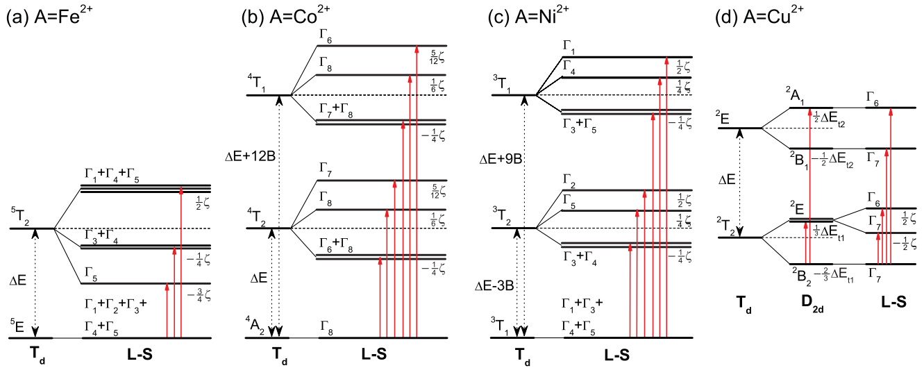
FIG. 10. (Color online) Energy-level diagrams corresponding to Fe^{2+} , Co^{2+} , Ni^{2+} , and Cu^{2+} 3d orbitals occupied by holes. In these diagrams, only the spin-allowed single-particle excitations are shown, red arrows represent the allowed optical transitions. (a), (b) 3d - 3d optical transitions within the d band of the A -site ion split by the cubic ( T_d ) crystal field \Delta E , the Racah parameter B , and the spin-orbit interaction \zeta for A = Fe^{2+} and A = Co^{2+} (Refs. 26 and 36). (c) In the case of A = Ni^{2+} , the effect of local T_d symmetry and spin-orbit interaction was taken into account, the latter as the weakest perturbation. Here, symmetry lowering associated with the weak tetragonal splitting was neglected. (d) In the case of A = Cu^{2+} , the effect of Jahn-Teller distortion, i.e., tetragonal splitting, \Delta E_1 was considered stronger than the spin-orbit interaction.
