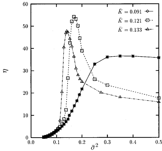
FIG. 45. The mean excess firing rate shown as a function of the variance of the noise \bar{\sigma}^2 for \lambda=0.1 , \bar{\gamma}=0.5 , and A_0=0.3 at three different values of the coupling K .
