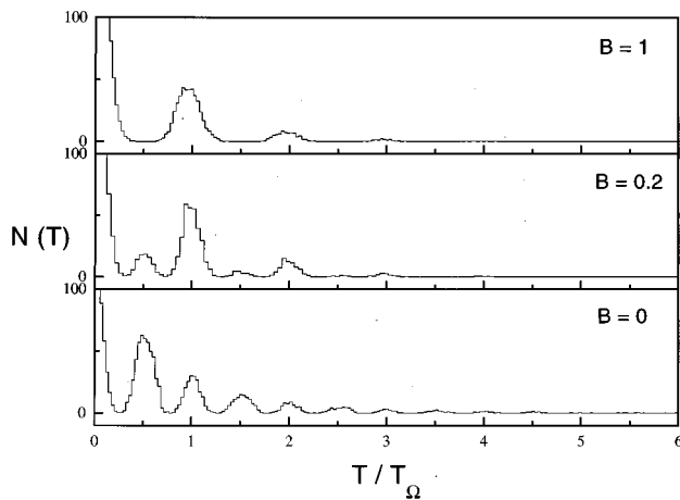
FIG. 13. Simulated residence-time distribution N(T) for the system of Eqs. (4.69) and (4.70) with \nu_\Omega=40 Hz, A_0=1 , and different values of B . Other circuital parameters are a=2 \times 10^4 s ^{-1} , x_m=1 , and D=0.16\Delta V . After Gammaitoni, Marchesoni, and Santucci (1994).
