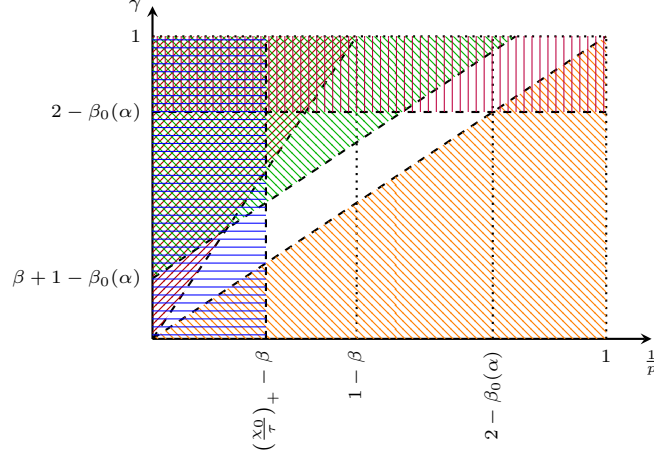
FIGURE 1. The white area contains all values (\gamma, 1/p) that satisfy (??).
