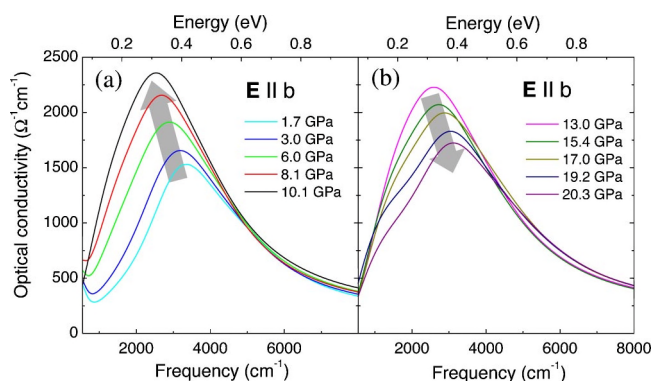
FIG. 3. (Color online) Pressure-dependent optical conductivity spectra of \beta\text{-Na}_{0.33}\text{V}_2\text{O}_5 at room temperature for the polarization \mathbf{E} \parallel b , obtained by Drude-Lorentz fits of the reflectivity data.
