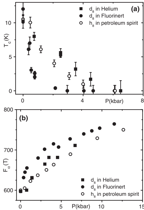
Figure 2. (a) T_c and (b) the \alpha -frequency, F_\alpha(T) , as a function of pressure for \kappa -( d_8 -BEDT-TTF) _2 Cu(SCN) _2 using helium (■) and using Fluorinert (●) [15] and for \kappa -( h_8 -BEDT-TTF) _2 Cu(SCN) _2 using petroleum spirit (○) [21] as a pressure medium.
