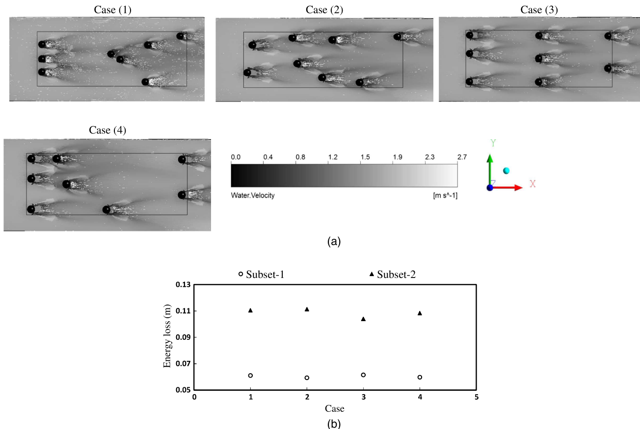
Fig. 11. Variation in energy loss for different spatial distributions, all other parameters remaining the same: (a) schematic for different spatial distributions; (b) energy loss variation
