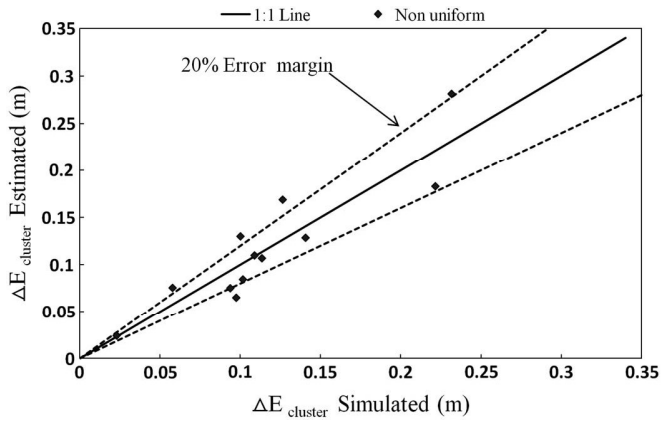
Fig. 14. Validation of empirical procedure for estimating energy loss due to cluster of nonuniformly sized boulders
