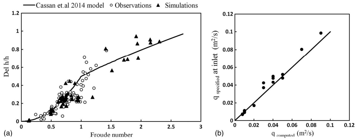
Fig. 7. Measured and simulated: (a) free surface deformation with Froude number; (b) validation Cassan Model [Eq. (12)]
