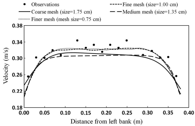
Fig. 2. Mesh sensitivity analysis; simulated streamwise velocities at x = 3.50 m and midheight
