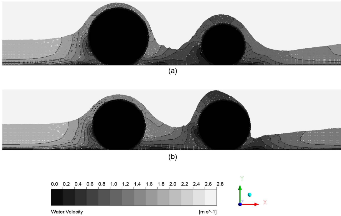
Fig. 16. Spatial variation of velocity on the central vertical plane: Run 125
