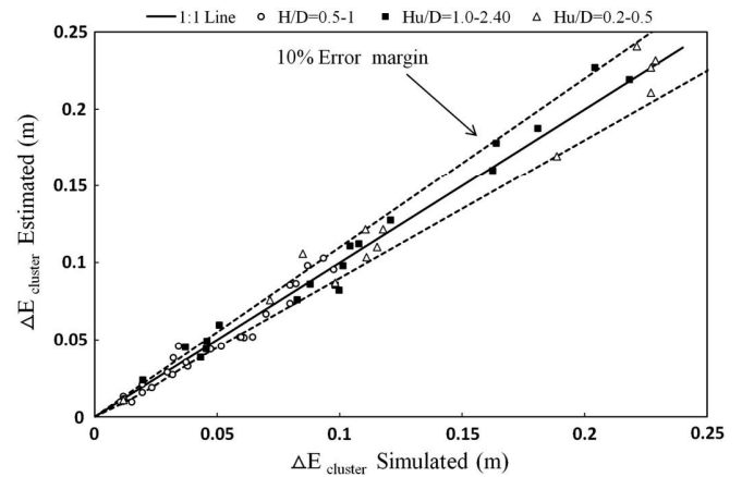
Fig. 13. Estimated and simulated energy loss for a cluster of boulders of uniform size
