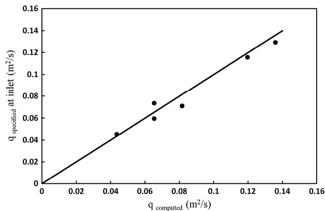
Fig. 6. Validation using flow resistance model proposed by Baki et al. (2014)
