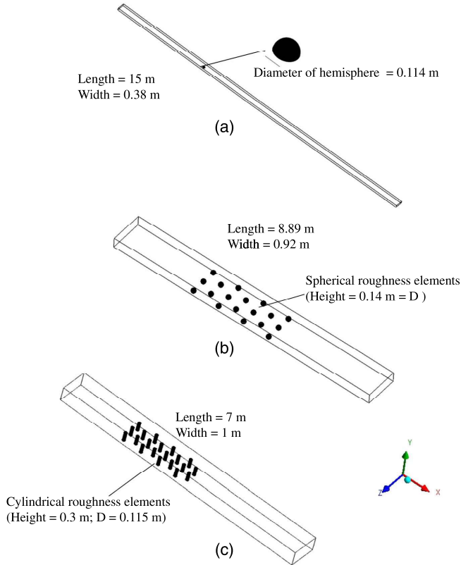
Fig. 1. Model domain for assessment of ANSYS-CFX package: (a) single hemispherical roughness element; (b) group of spherical roughness elements; (c) group of cylindrical roughness elements
