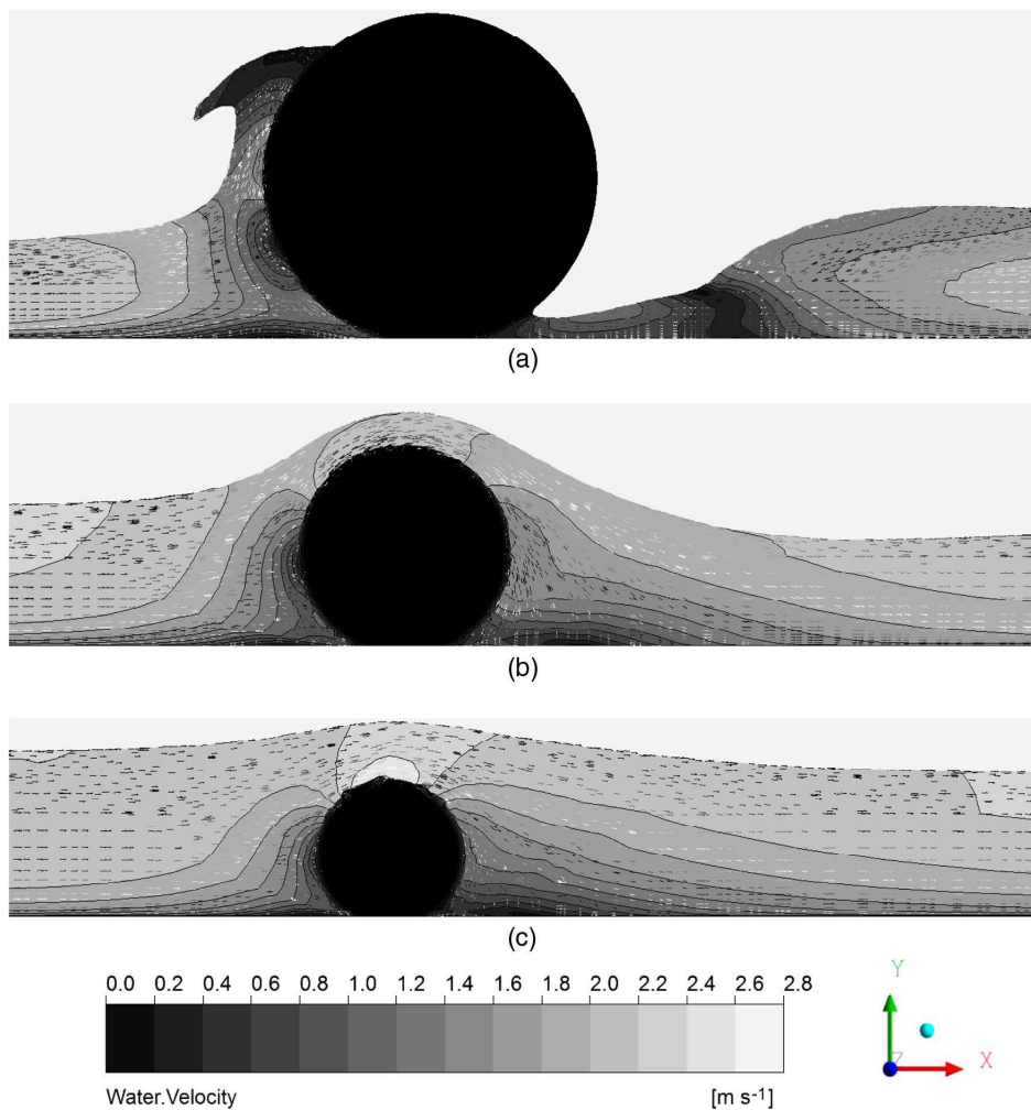
Fig. 8. Spatial variation of velocity on the central vertical plane for different cases of relative submergence (other conditions remain same): (a) Run 5; (b) Run 29; (c) Run 48
