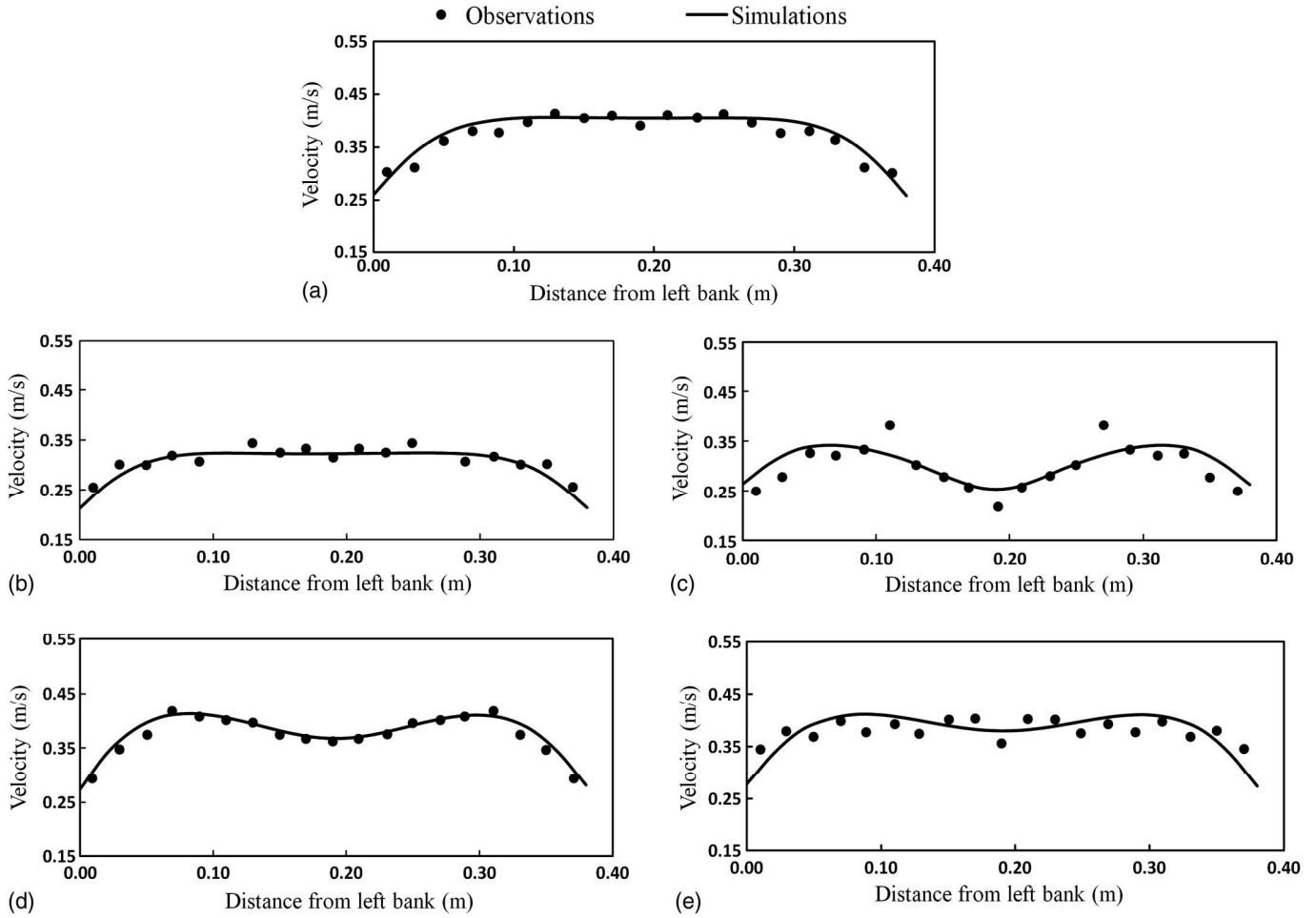
Fig. 4. Observed and simulated velocity profiles for Test Case 1: (a) uniform flow without the sphere; (b) at x = 3.5 m; (c) at x = 4.4 m; (d) at x = 5.5 m; (e) at x = 6.5 m
