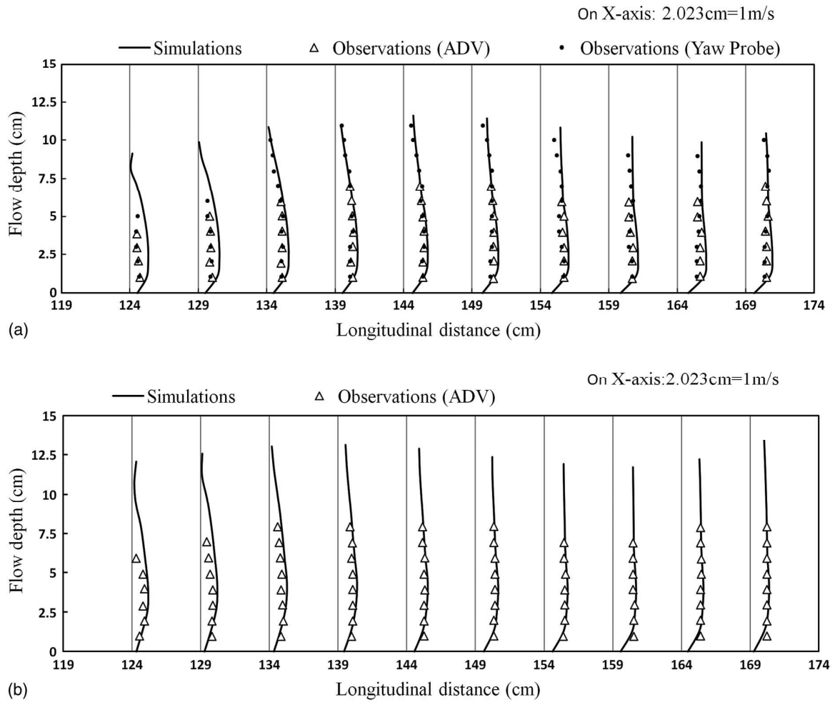
Fig. 5. Velocity profile comparison: (a) 0.06 m 3 /s flow rate and 5% bed slope; (b) 0.06 m 3 /s flow rate and 3% bed slope
