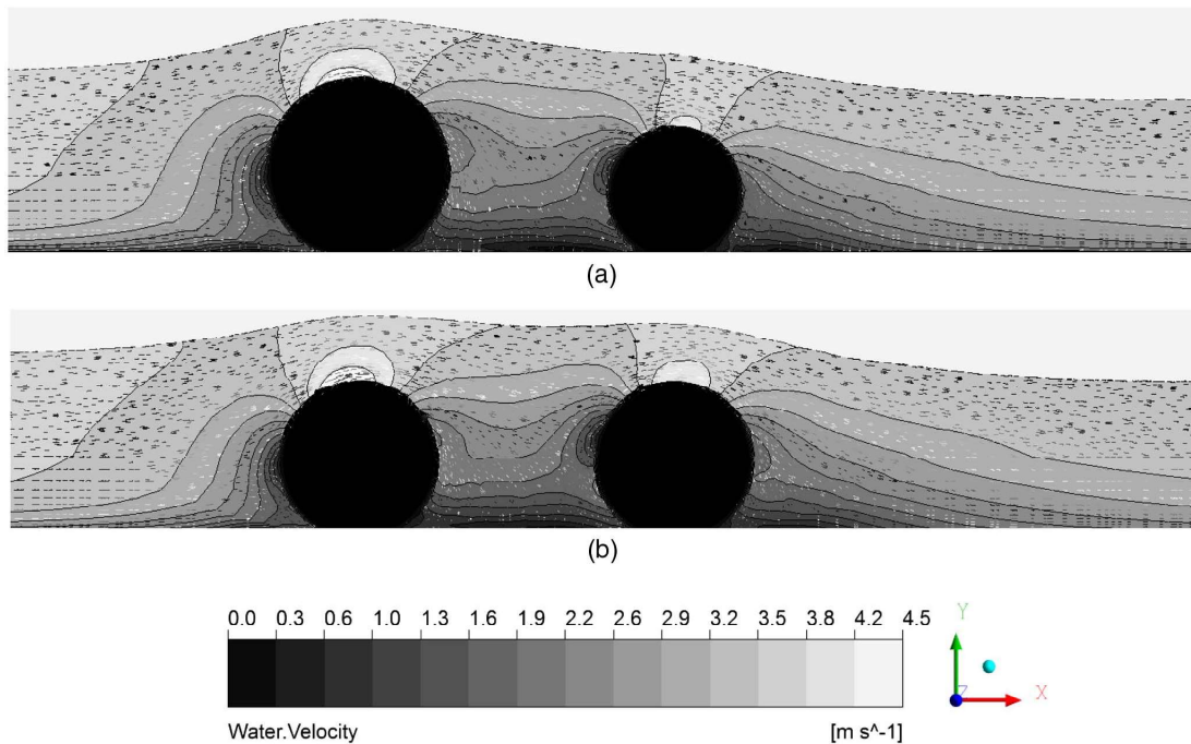
Fig. 15. Spatial variation of velocity on the central vertical plane: Run 124
