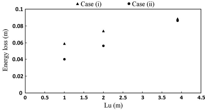
Fig. 9. Effect of boulder location on energy loss
