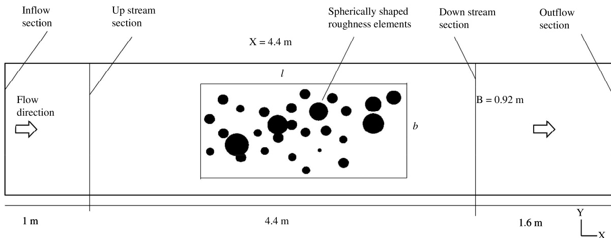
Fig. 3. Characteristic dimensions
