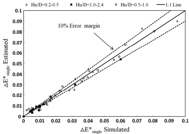
Fig. 10. Comparison of empirically estimated and numerically simulated energy losses
