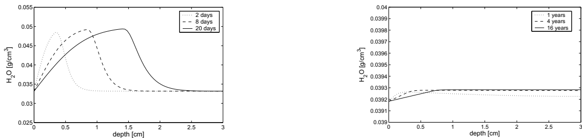
Figure 1: Numerical prediction of moisture profiles under accelerated and natural conditions. Left: Accelerated test, \text{CO}_2 = 50\% , \text{RH} = 65\% (cf. [PVF89]). Right: Natural test, \text{CO}_2 = 0.03\% , \text{RH} = 78\% (cf. [Wie84]).
