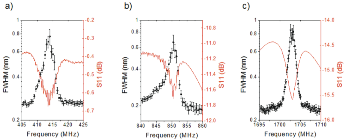
S-Fig. 1 – Broadening for three different SAW frequencies, f_{SAW} = 414 MHz (a), 850 MHz (b) and 1.7 GHz (c). The corresponding SAW wavelengths are \lambda_{SAW} = 28a , 14a and 7a , with a = 0.26 \mu\text{m} .
