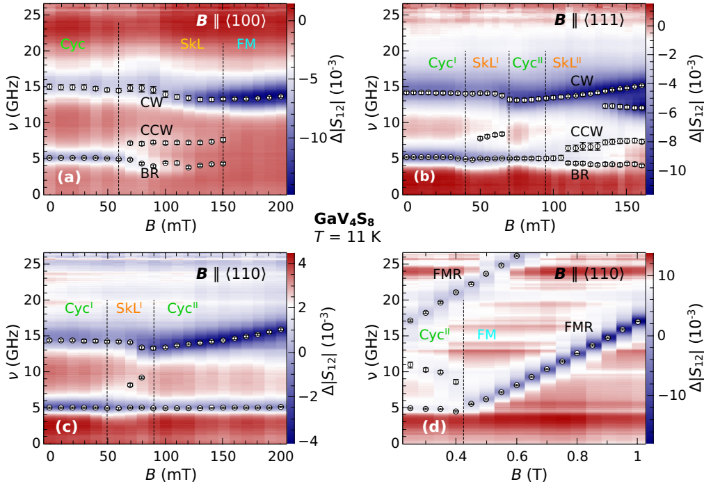
FIG. 4. (a)–(d) Color-coded plots of the transmission spectra \Delta|S_{12}| in the frequency vs magnetic field plane for T = 11 K for the field applied along the cubic principal directions. The intermediate white color has been shifted in order to emphasize weak amplitudes. Open circles with error bars are resonance frequencies from the Dysonian fits (see text). Dashed lines indicate transitions between cycloidal (Cyc), skyrmion lattice (SkL), and ferromagnetic (FM) phases. Panels (a)–(c) display low-field regimes, whereas panel (d) shows the spin-flop behavior at higher fields.
