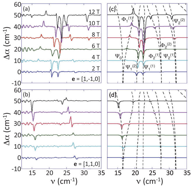
FIG. 5. (Color online) The measured [(a) and (b)] and predicted [(c) and (d)] NDD for 2 to 12 T fields along \mathbf{m} = [1, -1, 0] and for \mathbf{e} = [1, -1, 0] [(a) and (c)] or [1, 1, 0] [(b) and (d)]. Predictions are based on fit 2. Dashed curves in (c) and (d) are the predicted mode frequencies.
