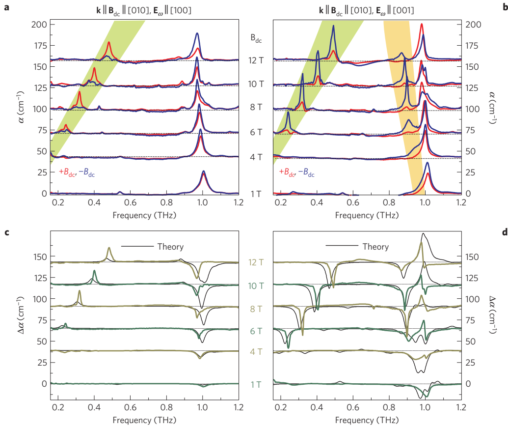
Figure 4 | Magneto-chiral effect in the field-induced chiral state. Absorption is studied when light propagates along the [010] axis parallel ( +B_{dc} ) and antiparallel ( -B_{dc} ) to the external magnetic field. a,b , Absorption spectra for light polarizations \mathbf{E}_\omega \parallel [100] ( a ) and \mathbf{E}_\omega \parallel [001] ( b ), measured as a function of the magnetic field, are shifted in proportion to the corresponding B_{dc} values. Red and blue curves indicate the case of +B_{dc} and -B_{dc} , respectively. Between the spin resonances the material is transparent, as \alpha \approx 0 . The magneto-chiral dichroism, corresponding to the difference of the absorption coefficients for counter-propagating beams, is huge both for the ‘Goldstone mode’ (highlighted green) and the low-frequency branch of the resonance at \sim 1 THz (highlighted orange). \Delta\alpha/\alpha_{\max} \gtrsim 70\% in the highlighted regions. c,d , The sign and magnitude of the experimentally observed MChD effect (coloured curves) are reproduced by our theoretical model (black curves) for two polarizations \mathbf{E}_\omega \parallel [100] and \mathbf{E}_\omega \parallel [001] as in c and d , respectively.
