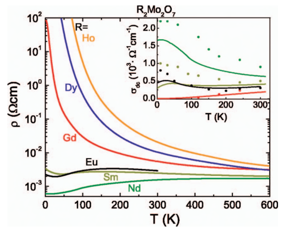
FIG. 2. (Color) Temperature dependence of the resistivity for six single crystals of \text{R}_2\text{Mo}_2\text{O}_7 . The inset shows the comparison of \sigma_{\text{dc}} and \sigma(\omega \rightarrow 0) below T=300 K for R=\text{Gd} , \text{Eu} , \text{Sm} , and \text{Nd} .
