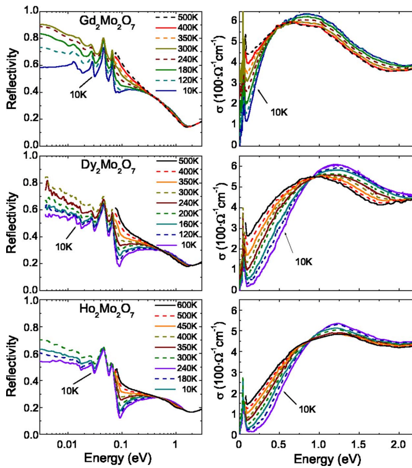
FIG. 6. (Color online) Reflectivity (left panel) and conductivity (right panel) spectra of the three insulators R=\text{Gd} , \text{Dy} , and \text{Ho} at selected temperatures.
