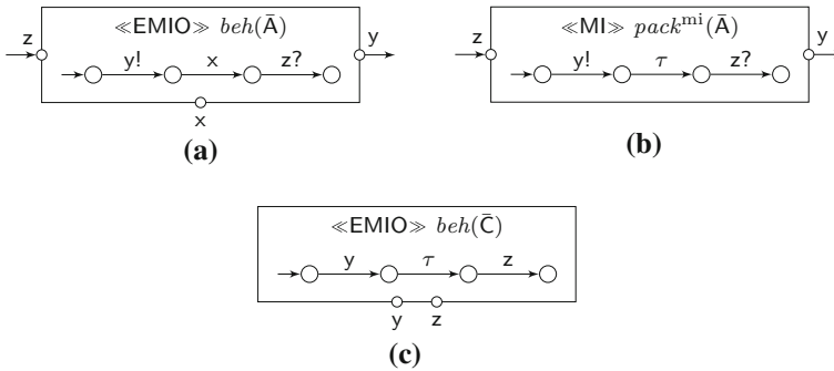
Fig. 9 Modal behaviours for assembly A in Fig. 6. a Behaviour of assembly \bar{A} . b Modal interface \text{pack}^{\text{mi}}(\bar{A}) . c Behaviour of assembly \bar{C}
