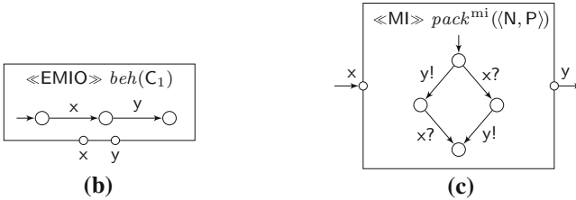
Fig. 11 Counter-example for (i). a Modal assembly C_1 . b Behaviour of assembly C_1 . c Modal interface pack^{mi}((N, P))
