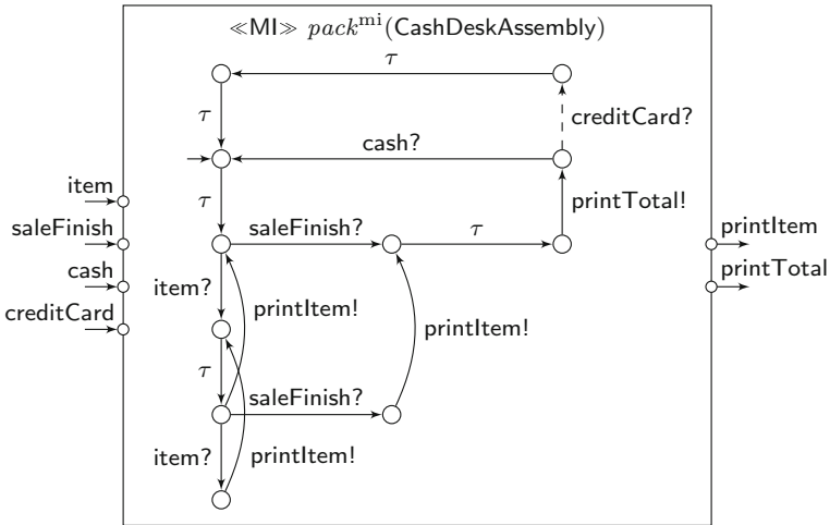
Fig. 17 Packed CashDeskAssembly
