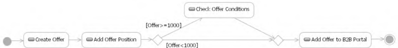
Fig. 4. Create Offer Process as Common Process Model
