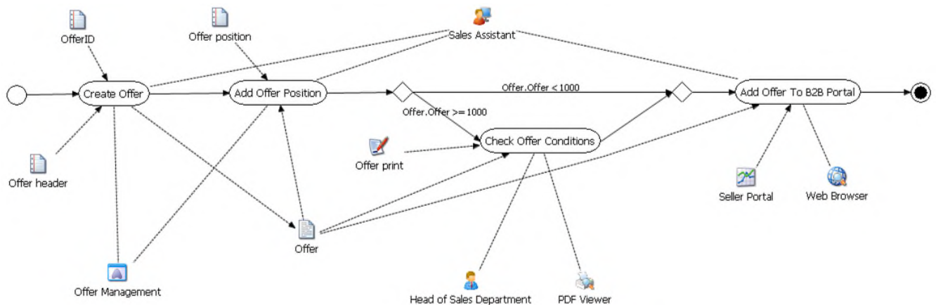
Fig. 1. Create Offer Process Modelled with AgilPro Light Modeller
