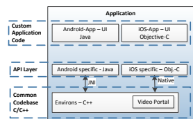
Figure 5: 3-layer architecture of Environs exemplified for the Google Android and Apple iOS platforms.
