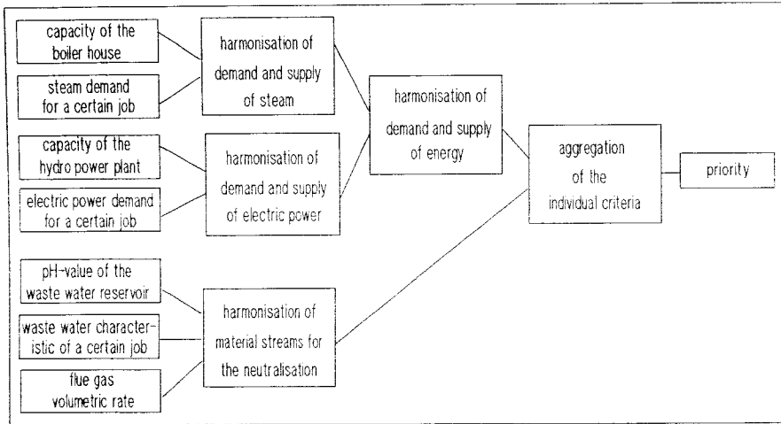
Figure 2: Structure of a Fuzzy Expert System for controlling energy and material flows
