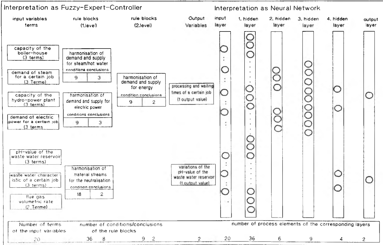
Figure 4: Interpretation of the Neuro-Fuzzy-System as Fuzzy Expert Controller and Neural Network
