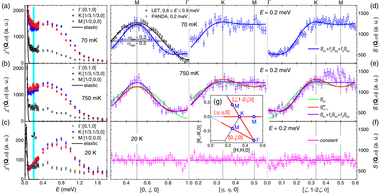
FIG. 2. Triple-axis INS data of \text{YbMgGaO}_4 measured on PANDA. Transfer-energy dependence of the dynamical spin susceptibility [25] measured at (a) 70 mK, (b) 750 mK, and (c) 20 K, at different high-symmetry \mathbf{Q} points. The black lines show the Gaussian fits to the elastic signal at the \Gamma point at -0.05 \leq E \leq 0.05 meV. Wave-vector dependence of the dynamical spin-correlation function [25] measured at (d) 70 mK, (e) 750 mK, and (f) 20 K, at the transfer-energy of 0.2 meV. The colored lines present the combined fits to the PANDA data using different model functions (see main text). High-energy ( 0.6 \leq E \leq 0.9 meV) LET data [25] are shown along [0, \xi, 0] in (d) for comparison, both the low and high energy full widths at half maximum (FWHM) are marked. (g) \mathbf{Q} scans. The red lines show the high-symmetry directions with special \mathbf{Q} points labeled, and the black lines represent Brillouin zone boundaries.
