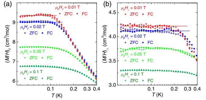
FIG. 1. Low- T magnetization data of YbMgGaO 4 measured at selected fields applied (a) parallel and (b) perpendicular to the c axis. The red and blue lines show the zero-temperature limits for the 0.01 and 0.02 T data, respectively.
