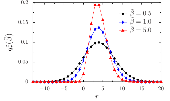
FIG. 5. (Color online) Probabilities q_r^c(\tilde{\beta}) for a canonical initial state as functions of r for |z|=2 and different values of the dimensionless inverse temperature \tilde{\beta}=0.5 (circles), 1 (diamonds), and 5 (triangles). The lines serve as a guide for the eye.
