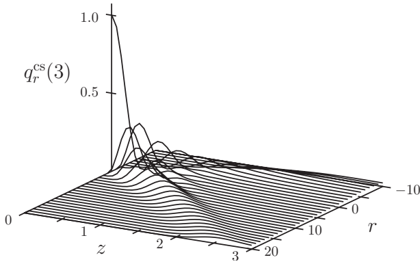
FIG. 6. Probabilities q_r^{cs}(\alpha) for a coherent state with parameter |\alpha|=3 for r=-10, \dots, 20 as functions of z .
