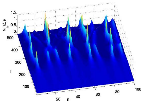
Fig. 1. Spatio-temporal evolution of the energy distribution E_n(t) . Initially the coordinates are uniformly distributed in the interval |q_n(0) - q_0| \leq \Delta q with mean q_0 = 0.45 and width \Delta q = 0.01 and p_n(0) = \Delta p = 0 . This leads to a total energy E_{\text{total}} = 17.2 \equiv 12.9 \times \Delta E . The parameter values are given by a = 1 , \omega_0^2 = 2 , N = 100 and \kappa = 0.3 .
