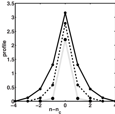
Fig. 3. Amplitude profile of the critical chain configuration for different coupling strengths: k = 0.1 ( dashed-dotted line ), k = 0.5 ( dashed line ), and k = 1 ( solid line ). For better illustration only the part of the lattice chain around the central site n_c with seizable elongations of the bonds is shown.
