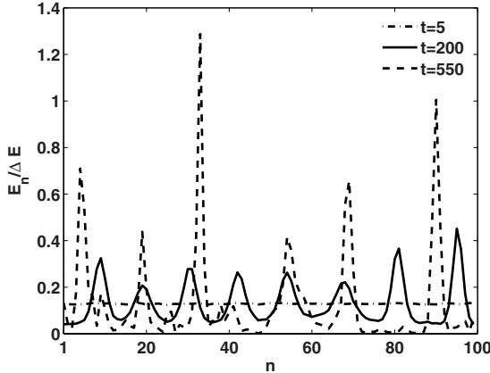
Fig. 2. Snap shots of the energy density at instants of time as indicated in the plot. Initial conditions: q_0 = 0.45 , \Delta q = 0.01 , p_0 = \Delta p = 0 . Parameter values: \omega_0^2 = 2 , a = 1 , N = 100 and \kappa = 0.3 .
