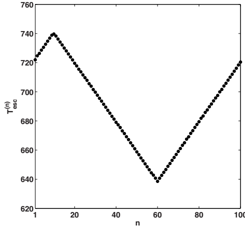
Fig. 4. The escape time of the chain units versus position. Initial conditions: q_0 = 0.45 , \Delta q = 0.01 , p_0 = \Delta p = 0 . Parameter values: a = 1 , \omega_0^2 = 2 , N = 100 and \kappa = 0.3
