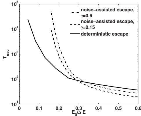
Fig. 5. Mean escape time as a function of the ratio E_0/\Delta E (for details see text) for the microcanonical ( solid line ) and Langevin ( dashed line and dashed-dotted line ) dynamics respectively. Parameter values: N = 100 , \omega_0^2 = 2 , a = 1 , \kappa = 0.3 and \gamma as given in the legend.
