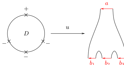
FIGURE 10.1. Disks u : (D, \partial D) \rightarrow (\mathbb{R} \times S^*Q, \mathbb{R} \times \Lambda_K) in the symplectization.
