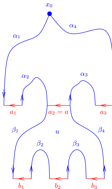
FIGURE 6.1. The definition of \partial(u) and \partial(u) \cdot_i \mathbf{a} .
