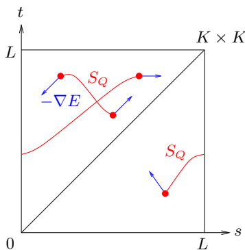
FIGURE 7.4. The space of 2-gons.
