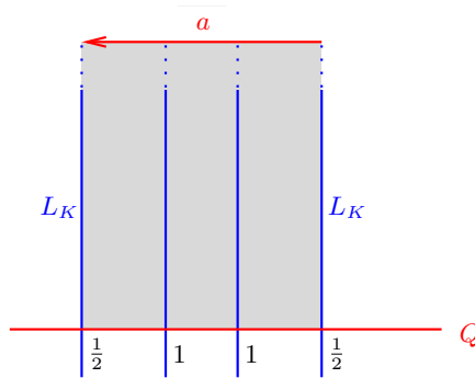
FIGURE 10.5. Curves with |\mathbf{n}| = 2 .
