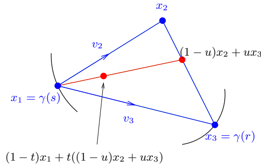
FIGURE 7.1. Parametrization of a triangle.
