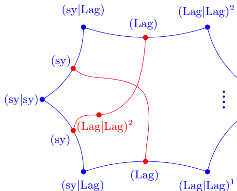
FIGURE 6.10. The 2-dimensional moduli space \mathcal{M}(a; \mathbf{n}) and the immersed curve \pi(\delta.\mathcal{M}(a; \mathbf{n})) .
