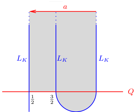
FIGURE 10.4. Curves with |\mathbf{n}| = 2 .
