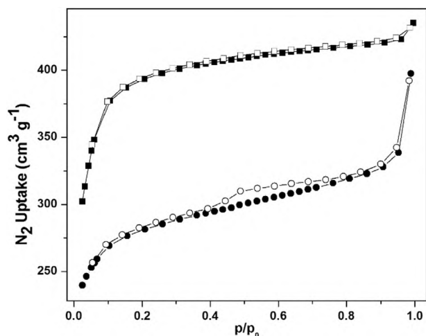
Fig. 5. \text{N}_2 adsorption (filled symbols) and desorption (empty symbols) isotherms of 1' (circles) and 2' (squares) measured at -196\text{ }^\circ\text{C} .
