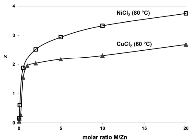
Figure 2. Total number, x , of Ni II or Cu II ions per \{M_xZn_{5-x}Cl_4\}^{6+} unit as a function of (M/Zn) molar ratio in the starting reaction mixture (DMA, 20 h).
