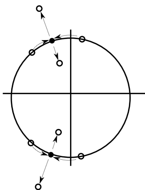
Figure 4.4. Collision of eigenvalues
