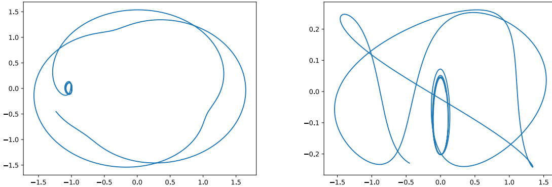
Figure 4.16. An orbit starting close to the periodic polar orbit: it shifted by about 400 km in the y -direction (orbits are fairly stable under shifts in the x -direction), and followed for five periods of the polar orbit.
