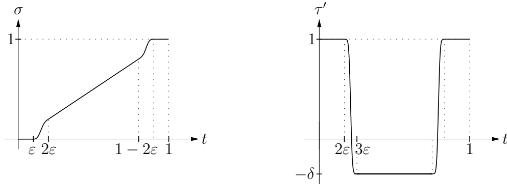
FIGURE 1. The graphs of \sigma and \tau' .
