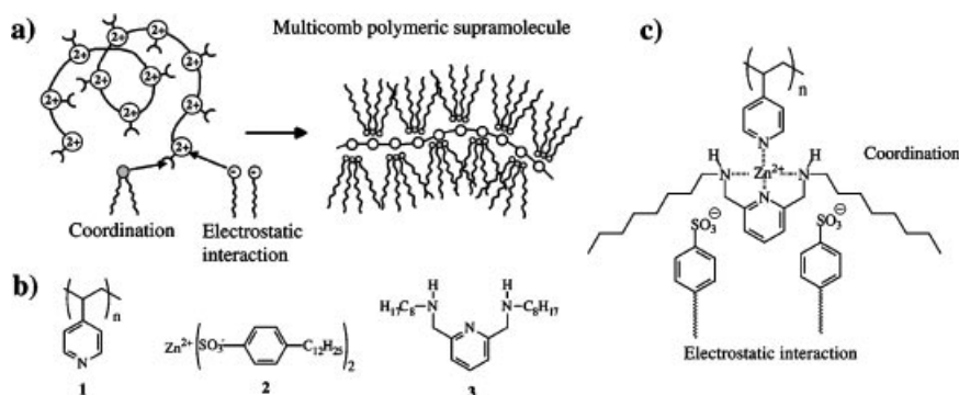
Fig. 4 (a) Multicomb polymeric superstructures derived from a polymeric backbone (1) and metal ion coordination of counter ions (2) and amphiphilic ligands (3). (b) Modules: P4VP (1), Zn(DBS) 2 (2), and 2,6-bis(octylaminomethyl)pyridine (3). (c) Suggested complexation with a 1:1:1 molar mixture of 1, 2, and 3 to form the polymeric metallosupramolecular poly[(4VP)Zn(2,6-bis(octylaminomethyl)pyridine)(DBS) 2 ]. (Adapted from ref. [63]).
