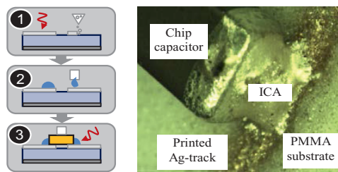
Figure 10: Interconnection of SMT components by ICA; left: (1) printing of the circuit pattern; (2) dispensing binder; (3) component placement and ICA curing; right: chip capacitor interconnected by light beam cured ICA.
