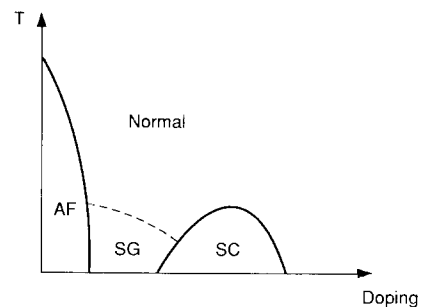
Fig. 1. A schematic phase diagram of the cuprate superconductors. AF, antiferromagnetic; SG, spin glass; SC, superconducting. x is the hole concentration.
