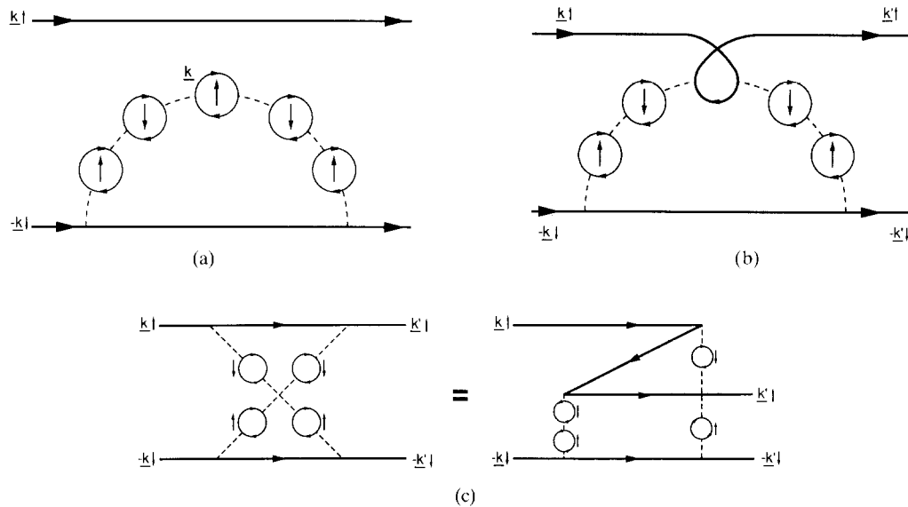
Fig. 5. Lowest order spin bag contribution to the pairing interaction.
