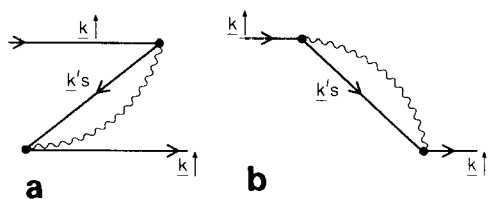
Fig. 2. ‘‘Backward’’ a) and ‘‘forward propagation’’ time-ordered Feynman diagram b). a) represents the contribution from the suppression of vacuum fluctuations and b) represents the spin-polaron contribution. s is up or down corresponding to the spin-flip or non spin-flip susceptibility, respectively.
