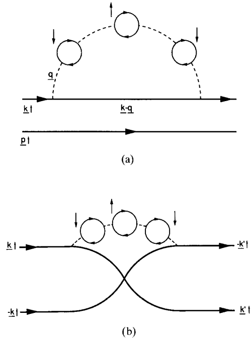
Fig. 4. Self-energy diagram in the presence of a second injected particle a); exchange diagram restoring the Pauli principle b).
