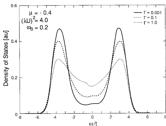
Fig. 3. Density of states as calculated from the model susceptibility for different values of \Gamma .
