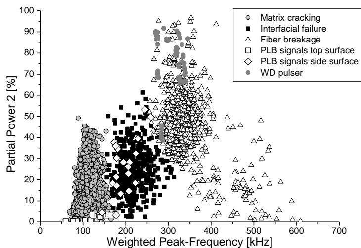
Figure 8: Comparison of position of signal features from AE test sources and measurement data from DCB test.
