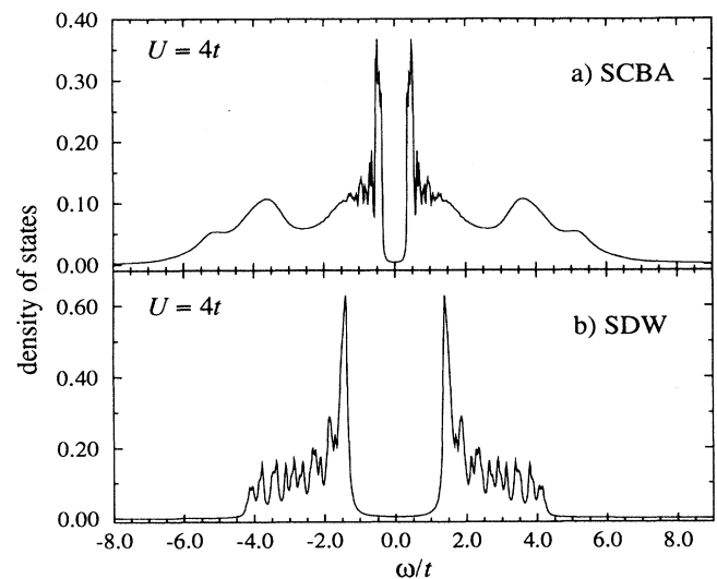
FIG. 5. Comparison of the density of states as obtained from the SCBA spectra for U = 4t on a 20 \times 20 lattice (a) with the bare SDW density of states for the same parameters (b).
