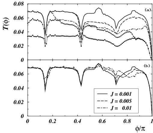
FIGURE 4. (a) Transmittance as a function of flux for a system of L = 8 with J = 0.001t_r , N + 1 = 8 particles and different window sizes ranging from 0.6t to 0.15t (top to bottom) below the Fermi energy. (b) as (a) for a selection of values of J .
