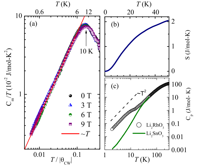
FIG. 2. (a) Magnetic heat capacity coefficient ( C_m/T ) in various fields as a function of T/|\theta_{\text{CW}}| . The upper axis shows the absolute T dependence and the solid line represents a T -linear fit, as discussed in the text. (b) T dependence of the magnetic entropy in zero field. (c) T dependence of the total heat capacity in zero field for \text{Li}_2\text{RhO}_3 compared with the nonmagnetic homologue \text{Li}_2\text{SnO}_3 . The dashed line indicates T^2 behavior.
