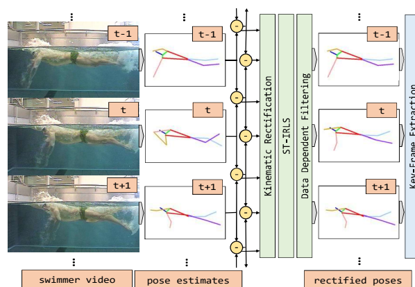
Figure 1: The proposed kinematic rectification pipeline (green) improves joint localization by enforcing temporal consistency between consecutive pose estimates.
