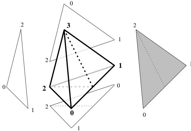
FIGURE 3. Local vertex numbering of submesh triangles along a 3d element of type 0 and positive orientation. As an example, the shaded triangle corresponds to the shaded box in Table 1.
