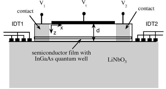
FIG. 1. The cross section of a hybrid semiconductor-piezocrystal structure. An epitaxial lift-off film has a thickness 0.5 \mu\text{m} . The Ohmic contacts are formed to a 2D electron gas. The transport gate with applied voltage V_t is used to control the conductivity of the electron plasma. A high-frequency (rf) signal is applied to the metal interdigital transducer IDT1 in order to generate surface acoustic waves. A surface acoustic wave propagates through a sample and is detected by the transducer IDT2.
