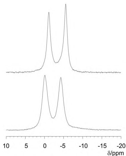
Figure 6. ^{31}\text{P}\{^{19}\text{F}\} CPMAS NMR spectra (no ^{19}\text{F} decoupling) for \text{Sr}(\text{PO}_3\text{F})\cdot\text{H}_2\text{O} (top) and \text{SrPO}_3\text{F} (bottom).
