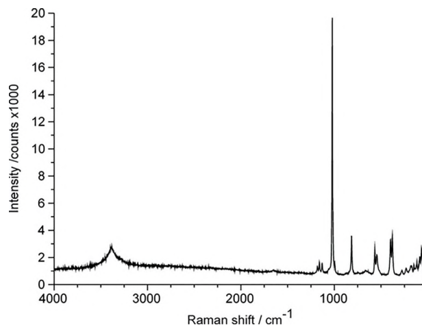
Figure 8. Raman spectrum of \text{Sr}(\text{PO}_3\text{F})\cdot\text{H}_2\text{O} .
