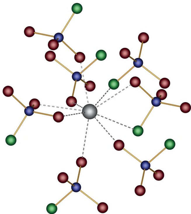
Figure 5. The coordination environment of the strontium ions in the crystal structure of \text{Sr}(\text{PO}_3\text{F}) ; the colour scheme is the same as that used in Figure 1.
