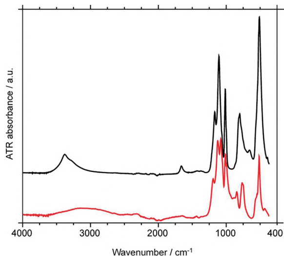
Figure 7. ATR infrared spectra of \text{Sr}(\text{PO}_3\text{F})\cdot\text{H}_2\text{O} (black) and \text{Sr}(\text{PO}_3\text{F}) (red; dried in air at 115 ^\circ\text{C} for two weeks).
