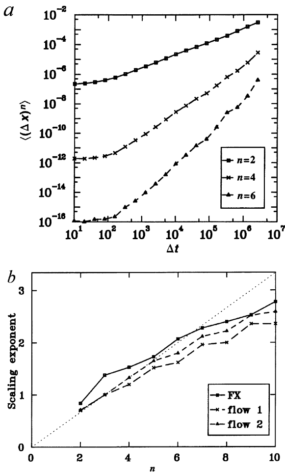
FIG. 2 a, Scaling of moments \langle (\Delta x)^n \rangle with n = 2, 4 and 6 . b, n -dependence of the scaling factors \xi_n and \zeta_n for the n th moments of the probability densities of FX price changes (squares) and hydrodynamic velocity differences taken from ref. 22 (crosses) and ref. 23 (triangles). Note the same qualitative deviation of all curves from a straight line.
