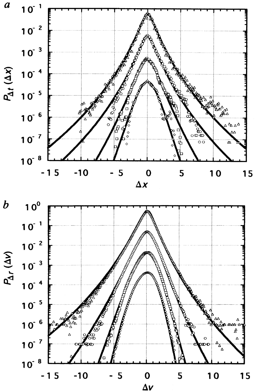
FIG. 1 a, Data points: standardized probability density P_{\Delta t}(\Delta x) of price changes \Delta x = x(t) - x(t + \Delta t) for time delays \Delta t = 640 s, 5,120 s, 40,960 s, 163,840 s (from top to bottom). The middle prices x(t) = (x_{\text{bid}}(t) + x_{\text{ask}}(t))/2 have been used (data provided by Olsen & Associates (see text)). The probability density has been calculated in a similar way as ref. 10. Full lines: results of (least-squares) fits carried out according to ref. 7; \lambda^2 = 0.25, 0.23, 0.13, 0.06 (from top to bottom). For better visibility, the curves have been vertically shifted with respect to each other. Note the systematic change in shape of the densities. b, Data points: standardized probability density P_{\Delta r}(\Delta v) of velocity differences P_{\Delta r}(\Delta v) for a turbulent flow with \Delta r = 3.3\eta, 18.5\eta, 138\eta, 325\eta (data taken from ref. 13, R_i = 598 . Here \eta is the Kolmogorov scale, where viscous dissipation occurs. Full lines: results of (least-squares) fits carried out according to ref. 7; \lambda^2 = 0.19, 0.10, 0.04, 0.01 .
