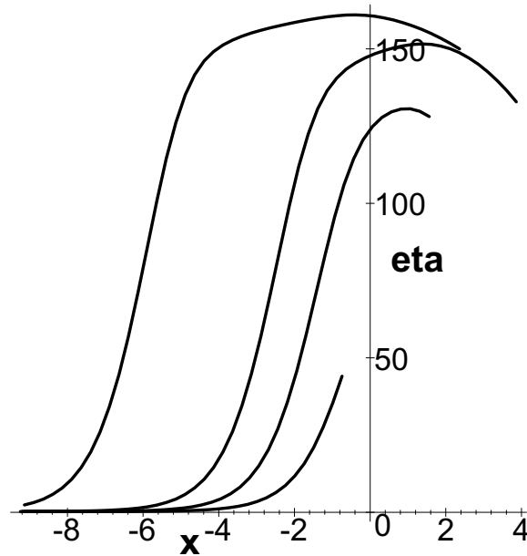
Figure 8. Spectral amplification as a function of the scaled noise strength x = -\ln(\sqrt{(2)\Omega}) - \beta/4 for A = 0.1 and different driving frequencies \Omega = 10^{-5} , \Omega = 10^{-4} , \Omega = 10^{-3} , and \Omega = 10^{-2} , from top to bottom. Only for the largest frequency the maximum is approximately located at x = 0 where it should be according to the T(\beta) = \sqrt{(2)\Omega} \exp\{\beta/4\} . The maxima for larger frequencies lie at substantially larger noise strengths.
