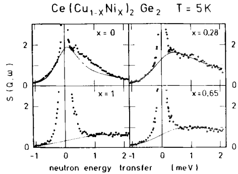
Fig. 12 Scattering law vs neutron-energy transfer for an average scattering angle \theta = 19 \text{ deg} as obtained in \text{Ce}(\text{Cu}_{1-x}\text{Ni}_x)_2\text{Ge}_2 for concentrations x = 0, 0.28, 0.65 and 1 at T = 5 \text{ K} . Solid lines are the results of fits using a Lorentzian line shape. Data for x = 0 , and x = 1 are taken from [7] and [8], respectively.
