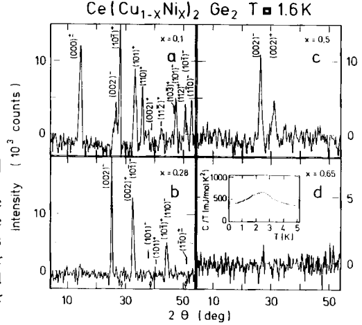
Fig. 10 Difference spectra [I(1.6 \text{ K}) - I(6 \text{ K})] for \text{Ce}(\text{Cu}_{1-x}\text{Ni}_x)_2\text{Ge}_2 with concentrations x = 0.1, 0.28, 0.5 and 0.65 : Bragg reflections shown are of magnetic origin only. The positions of the nuclear Bragg reflections are indicated by arrows in (b). For x = 0.1 , the (002)^+ satellite and for x = 0.28 the (101)^- , (101)^+ satellites are screened by nuclear Bragg peaks. Specific-heat results for x = 0.65 are given as C/T vs T in the inset of (d).
