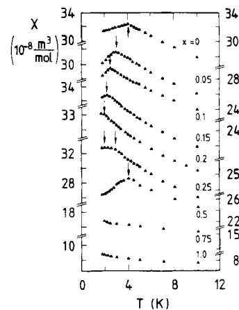
Fig. 3 DC susceptibility \chi vs T measured at B = 1 T for \text{Ce}(\text{Cu}_{1-x}\text{Ni}_x)_2\text{Ge}_2 with different Ni-concentrations, x . Arrows indicate Néel temperatures, cf. Fig. 2.
