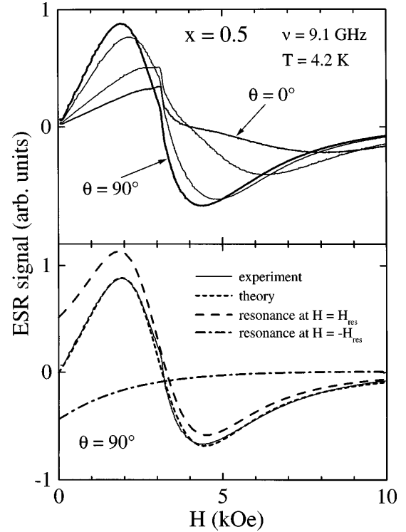
FIG. 2. Upper frame: ESR spectra from oriented powder samples of \text{Ce}(\text{Cu}_{0.5}\text{Ni}_{0.5})_2\text{Ge}_2 doped with 2% Gd for different orientations ( \vartheta=0^\circ, 30^\circ, 60^\circ, 90^\circ ) at 4.2 K. The distortions at 3.3 kOe originate from the background of the cavity. Lower frame: fit with a Dysonian line shape (short dashed) according to Eq. (1). The dashed and dash-dotted lines show the contributions of both circular polarization components as described in the text.
