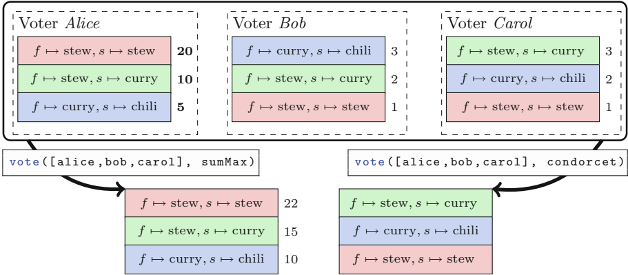
Fig. 1. Social welfare functions can reduce weight-induced bias. Agents pick meals for Friday f and Saturday s , with three solutions in \text{sols(CSP)} due to hard constraints. Alice submits manipulated weights which puts (f \mapsto \text{stew}, s \mapsto \text{stew}) to the top whereas the other agents like it least. Condorcet voting mitigates that by ranking (f \mapsto \text{stew}, s \mapsto \text{curry}) first since it wins both pairwise majority contests against the other solutions.
