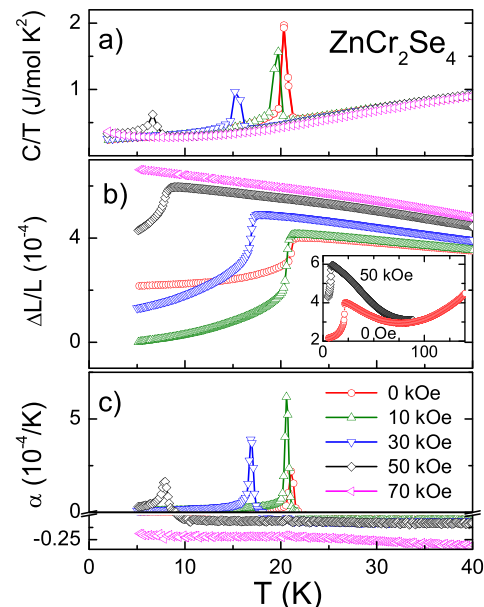
FIG. 2 (color online). (a) Temperature dependence of the heat capacity of a \text{ZnCr}_2\text{Se}_4 single crystal plotted as C/T vs T . (b) Relative length change of the sample \Delta L(T)/L_0 . Data are normalized to the monodomain state at H = 0 and T = 4.3 K. Inset: \Delta L(T)/L_0 for an extended temperature range illustrating the negative thermal expansion between T_N and 75 K in H = 0 and 50 kOe. (c) Thermal expansion \alpha at different magnetic fields between 0 and 70 kOe applied along the \langle 001 \rangle axis.
