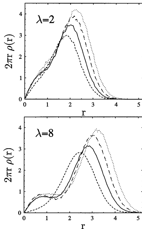
FIG. 1. Density \rho(r) of the spin-polarized state ( S = N/2 ) for \lambda = 2 (top) and \lambda = 8 (bottom). Dashed, solid, dash-dotted, and dotted curves correspond to N = 5, 6, 7 , and 8 , respectively. Units are such that l_0 = 1 .
