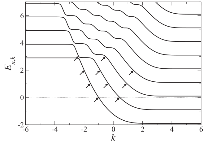
FIG. 11. Spectrum E_{n,k} vs k for a straight p - n junction of Schrödinger fermions. Energies (wave numbers) are in units of \omega_c ( l_B^{-1} ); cf. Eq. (2). The shown results are for V_0/\omega_c = 2.4 and follow from Eq. (A4). Density profiles are illustrated in Fig. 12 for the states with E_{n,k} = 0, 1, 2, 3 indicated by arrows.
