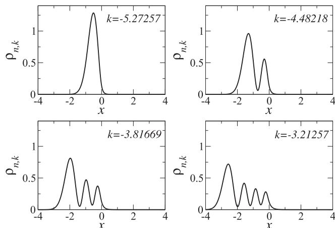
FIG. 3. Spatial profile of the probability density \rho_{n,k}(x) at V_0 = 2.4 for four different eigenstates with energy E_{n,k} = +2 and wave numbers k \simeq -5.27 , -4.48 , -3.82 , -3.21 . These states are indicated by green arrows in Fig. 2(c).
