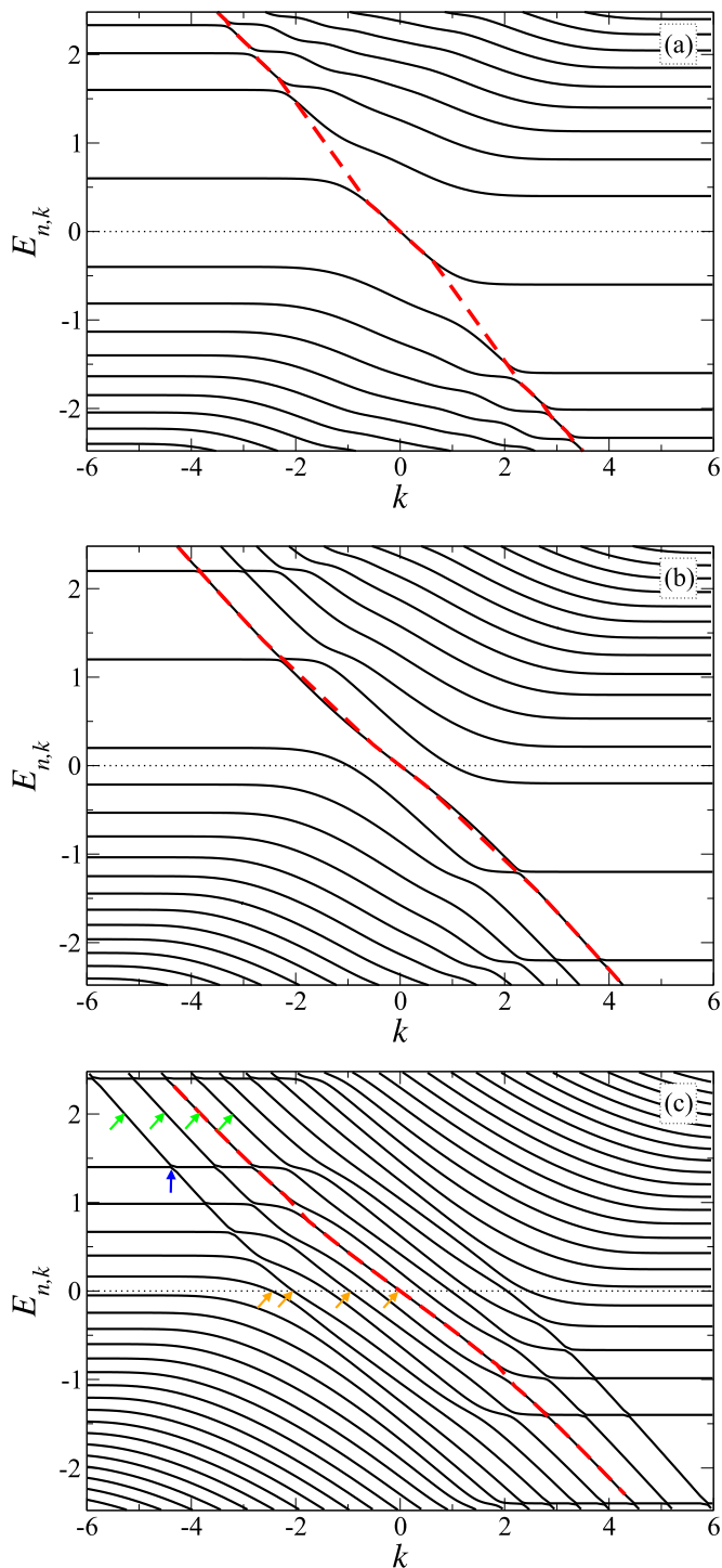
FIG. 2. Spectrum E_{n,k} vs k obtained from Eq. (12) for a straight p - n junction, with units in Eq. (2): (a) V_0 = 0.6 , (b) V_0 = 1.2 , and (c) V_0 = 2.4 . Red dashed curves are guides to the eye only and illustrate the central chiral interface state passing through k = E = 0 . Density profiles for the four E = 2 ( E = 0 ) states labeled by green (orange) arrows are shown in Fig. 3 (in Fig. 4). The blue vertical arrow shows the avoided crossing studied in Fig. 5.
