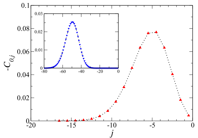
FIG. 10. Dimensionless coefficients -C_{n=0,j<0} vs j determining the ring currents in Eq. (31) for a circular p - n junction with R = 3.3 (main panel) and R = 10 (inset). The shown results follow from first-order perturbation theory in V_0 ; see Eq. (B5) in Appendix B. Dotted curves are guides to the eye only. In the inset, one clearly sees that the maximum of |I_{0,j}| in Eq. (31) is reached for half-integer j = j_0 \approx -R^2/2 = -50 .
