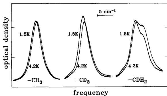
Fig. 4. The red edge zero-phonon origins of dimethyl-s-tetrazine and its deuterated derivative at 4.2 and 1.5 K.
