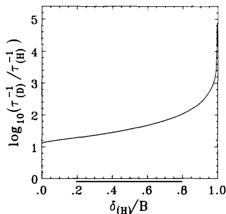
Fig. 7. Ratio of the conversion rates \tau^{-1} for deuterated (D) and protonated (H) methyl species versus the tunneling frequency \delta_{(H)} in units of the (protonated) rotational constant B of the protonated rotor, assuming a Raman process as conversion mechanism. This ratio is nearly temperature independent. It is assumed that the height V_3 of the orientational potential and the rotor-phonon coupling strength do not change with deuteration. For the ratio of the quadrupolar energy C_Q of a deuteron in the electric field gradient of a CD bond and the dipolar energy ( \gamma^2/r^3 ) between two protons in a methyl group a value C_Q/(\gamma^2/r^3) = 1.5 is assumed here.
