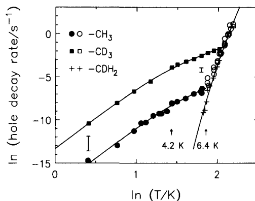
Fig. 5. Log-log plot of the hole recovery rate vs. temperature.
