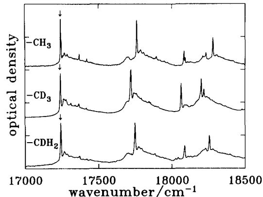
Fig. 2. Absorption spectrum of dimethyl- s -tetrazine in n -octane. Resolution: 1 cm -1 . Temperature: 4.2 K. Hole burning was performed at the red edge origin (arrows).
