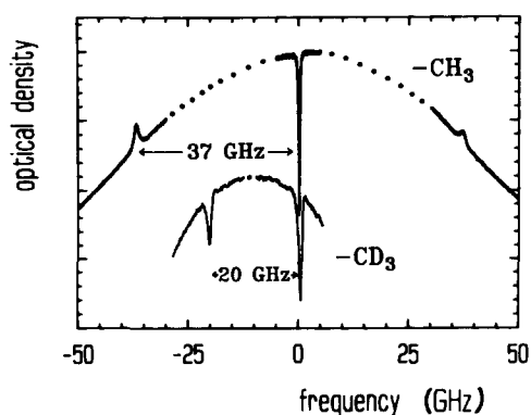
Fig. 3. Hole-antihole (side hole) splitting for dimethyl-s-tetrazine and its perdeuterated analogue in n-octane at 4.2 K.
