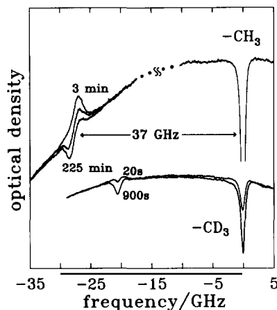
Fig. 6. Upper trace: the spectral range around the antihole in dimethyl-s-tetrazine at 4.2 K. Note that as the antihole decays, a side hole grows in, but the side hole is shifted. Lower trace: the same phenomenon as in the upper trace for the \text{CD}_3 derivative. The central hole is shown, too. The antihole is not as pronounced as in the upper trace, because at 4.2 K, relaxation in the \text{CD}_3 -tunneling states is fast.
