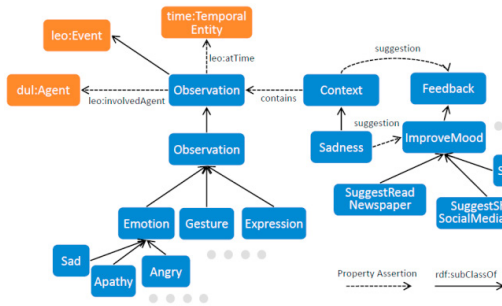
Fig. 4: Observation and Context models
